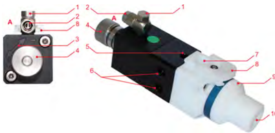
Fig. 1: Description: Metering valve EP-SV 295243
