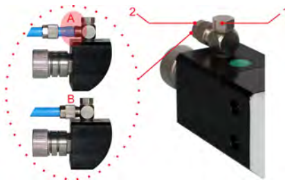
Fig. 3: Compressed air connection
