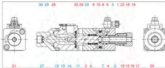
Fig. 6: Wear and spare parts for metering valve EP-SV 295243
