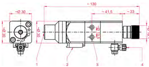
Fig. 8: Metering valve EP-SV 295243 dimensions
