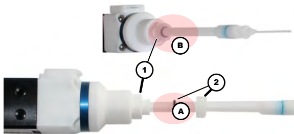
Fig. 4: Dosing connection with dosing tip extension and dosing tip
