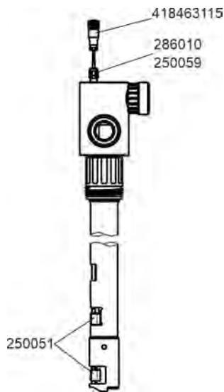
Fig. 8: Spare parts
