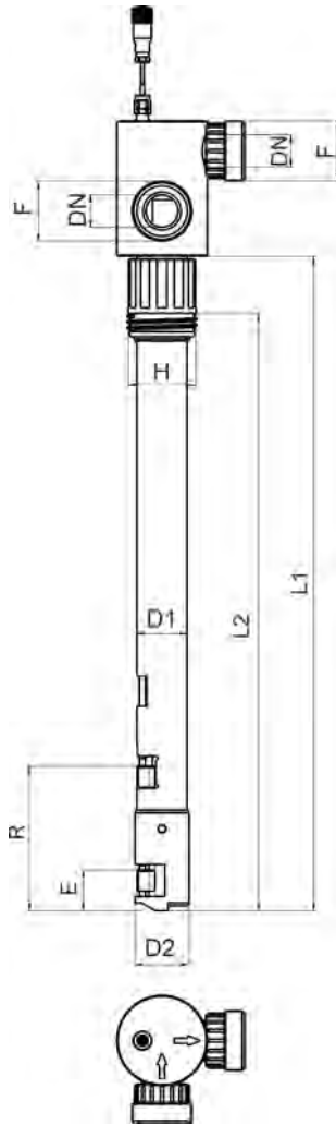
Fig. 7: Dimensions suction lance
