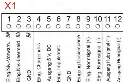
Fig. 7.17 Bornier X1
