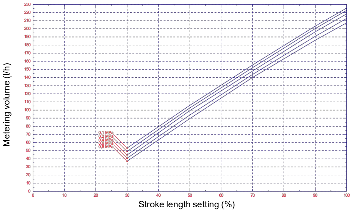
Fig. 14.5 Delivery capacity type 02100 / 0.8 MPa (8 bar)
