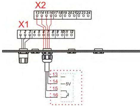
Fig. 7.27 Installation diaphragm burst detector
