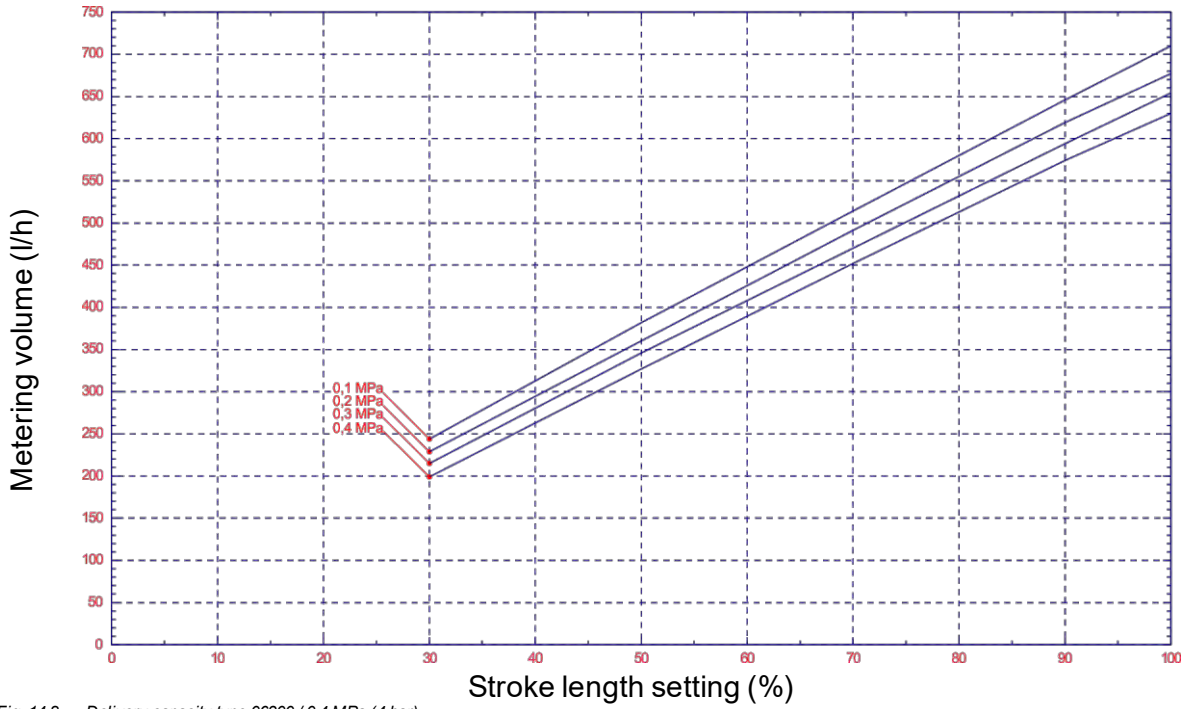
Fig. 14.8 Delivery capacity type 06300 / 0.4 MPa (4 bar)
