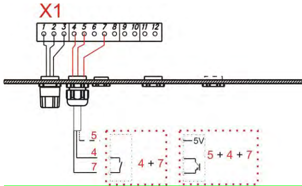
Fig. 7.23 Installing the batch function
