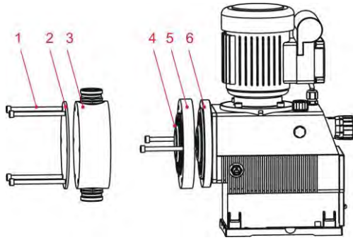
Fig. 11.4 Metering head and diaphragm replacement
