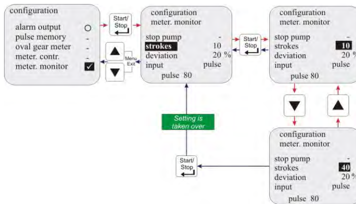
Fig. 10.36 Configuration / Metering monitoring / Strokes
