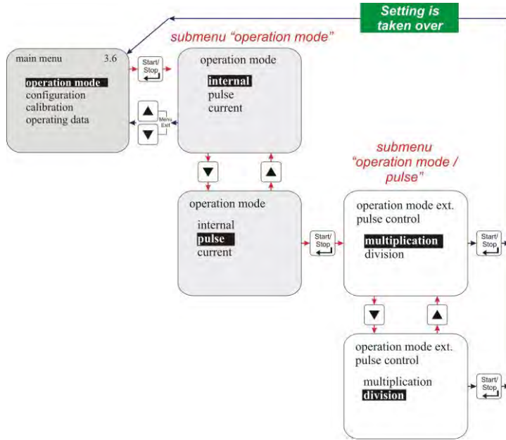
Fig. 10.8 Operation mode / pulse / selecting
