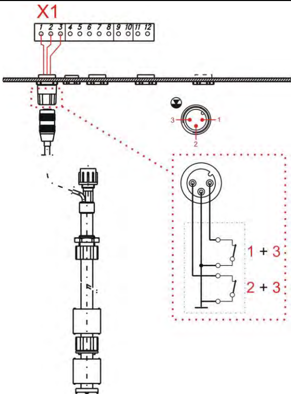
Fig. 7.19 Installing the suction pipe with low-level advance warning and empty report
