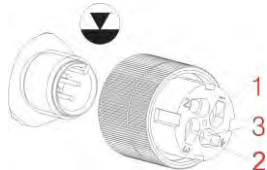
Fig. 14.2 Connector assignments: low-level advance warning
