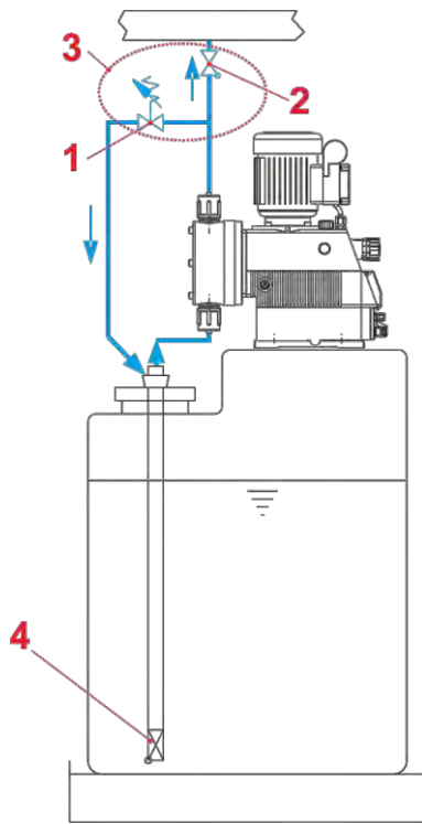
Fig. 6.1 Mounting diagram
