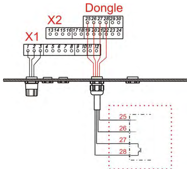
Fig. 8.3 Installation Oval Gear Meter
