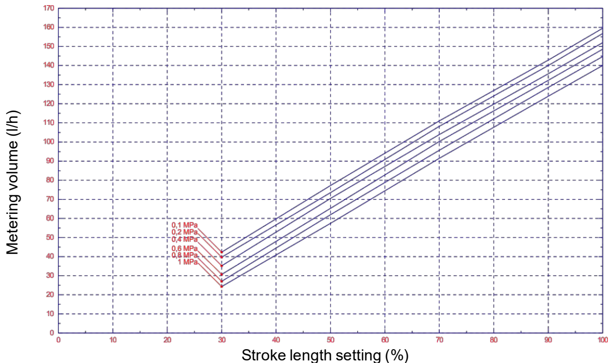
Fig. 14.3 Delivery capacity type 01400 / 1 MPa (10 bar)
