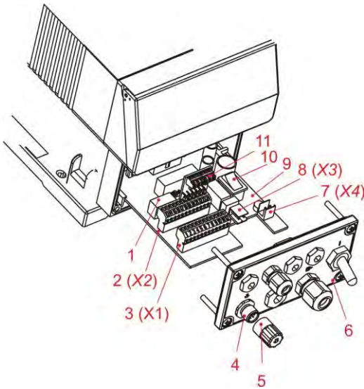
Fig. 7.15 Overview Control Board
