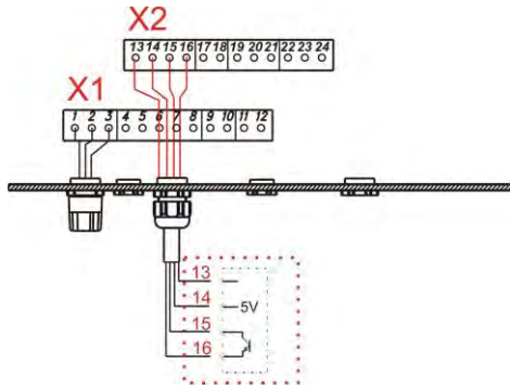
Abb. 7.27 Installation Membranbruchsensoren
