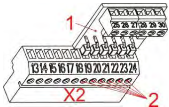
Fig. 8.1 Fitting the Dongle-Plate
