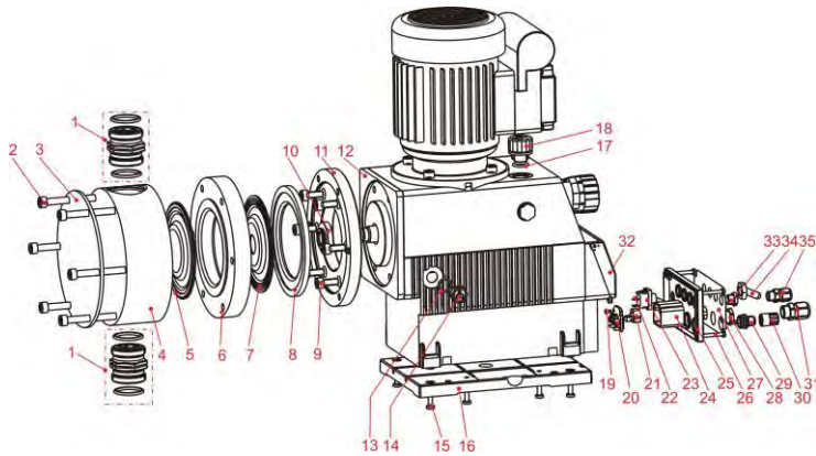
Fig. 13.1 Wearing parts and spare parts
