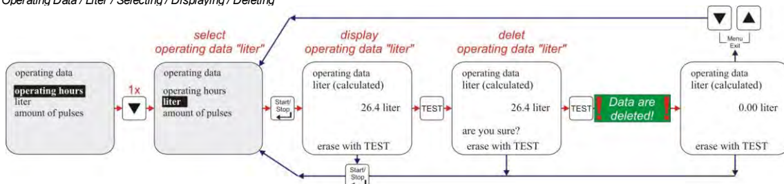
Fig. 10.54 Operating Data / Liter / Selecting / Displaying / Deleting
