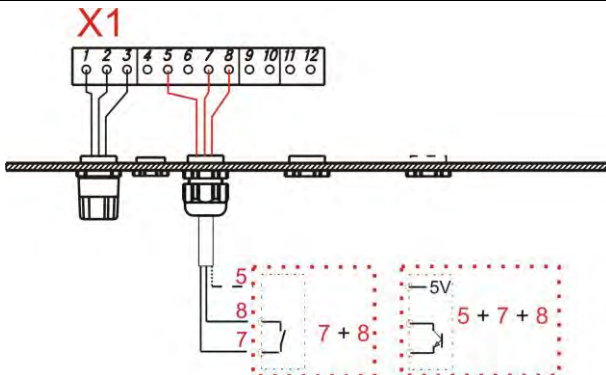
Fig. 7.22 Installing the control via metering lock
