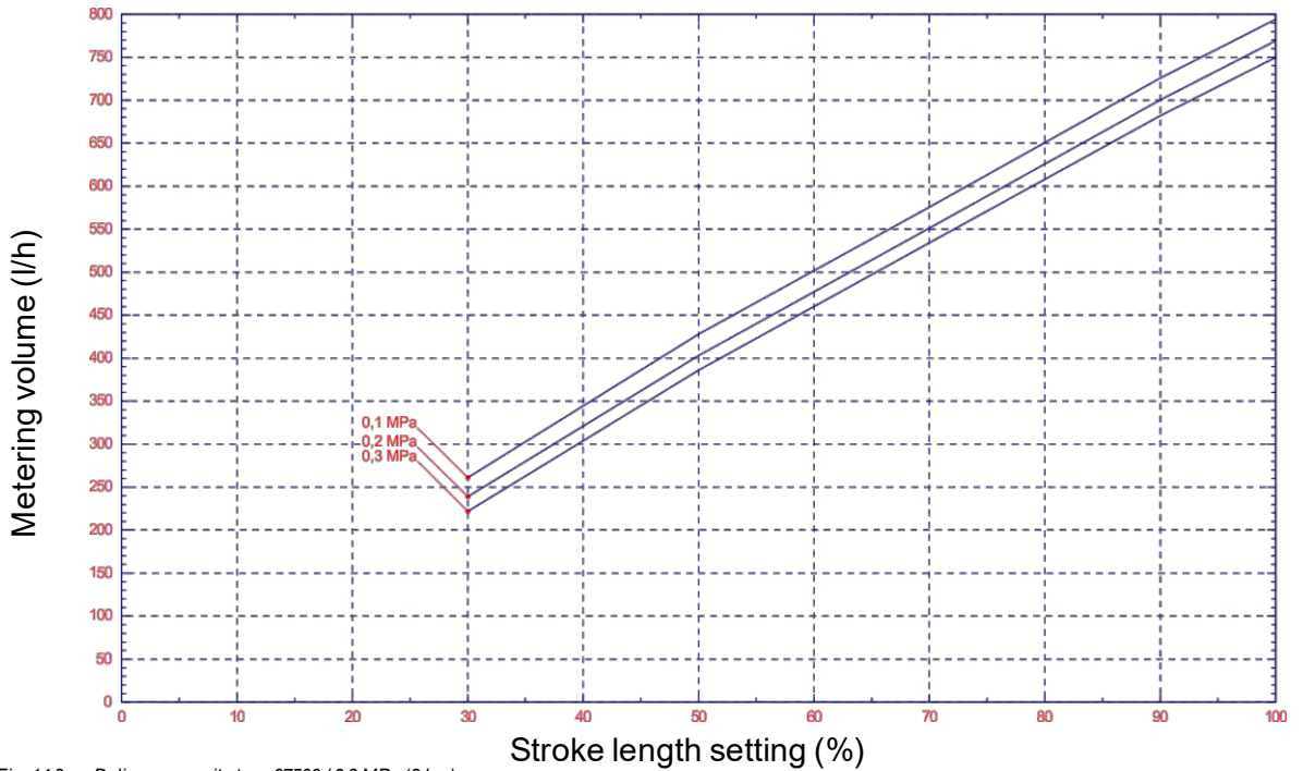
Fig. 14.9 Delivery capacity type 07500 / 0.3 MPa (3 bar)
