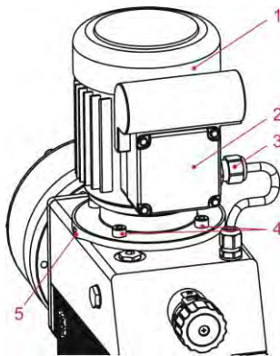
Fig. 11.6 Motor replacement
