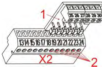
Abb. 8.1 Montage Dongle-Platine
