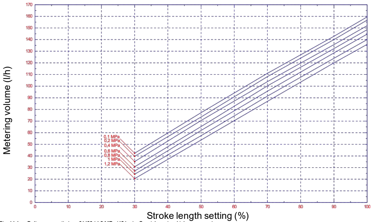
Fig. 14.4 Delivery capacity type 01400 / 1.2 MPa (12 bar) - Special version: higher pressure
