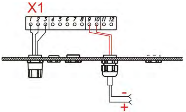
Fig. 7.21 Installing the standard signal control
