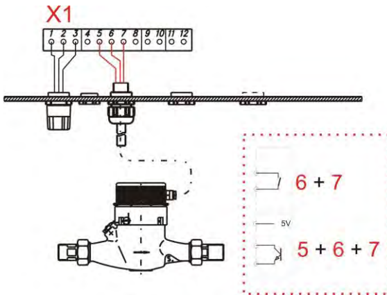
Fig. 7.20 Installing the pulse control (water meter)
