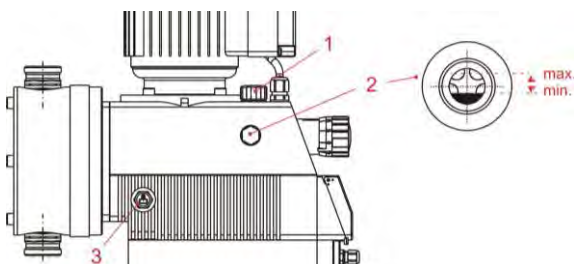
Fig. 11.5 Gear Oil Change
