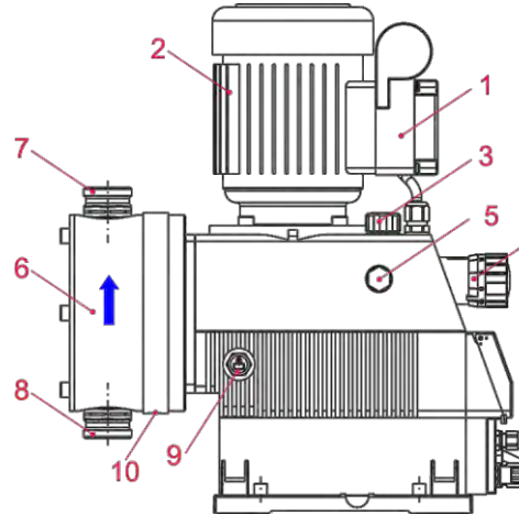
Fig. 5.2 EMP IV E60 (side view)
