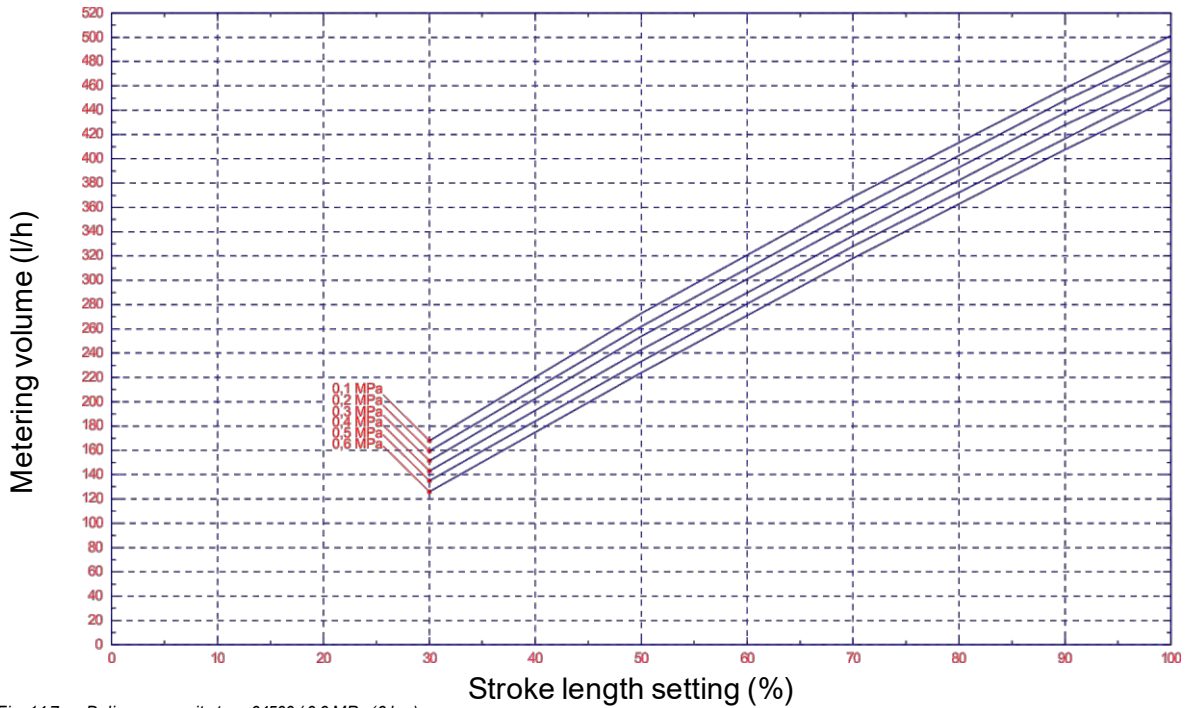
Fig. 14.7 Delivery capacity type 04500 / 0.6 MPa (6 bar)
