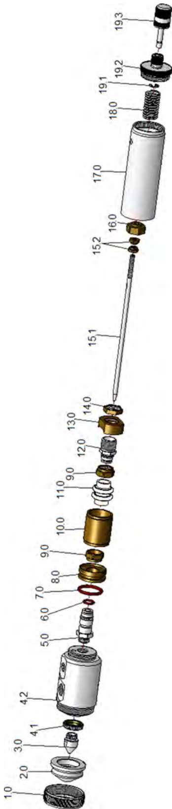
Fig. 8: Spare parts
