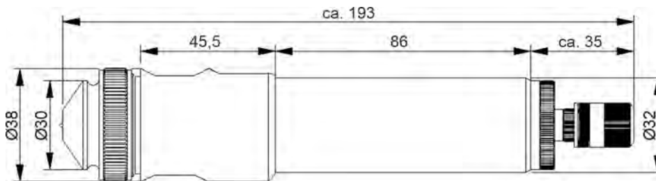
Fig. 9: Dimensions
